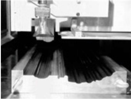
Profile grinding of large plates
