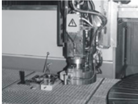
Straight/profile dressing of grinding wheel with table mounted dressing unit
